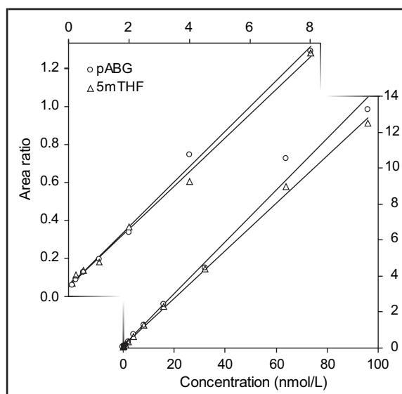
Fig. 3. Linear dynamic range for the pABG method.
